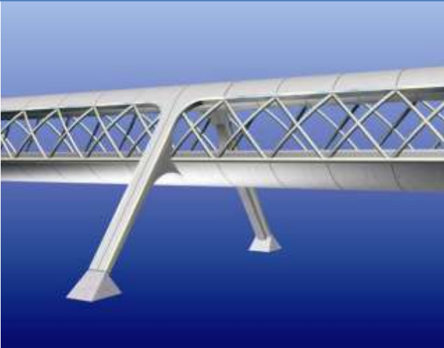
Preliminary designs for Dese viaduct in Italy (2007)
