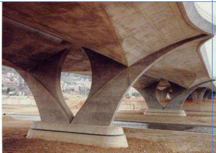
Bridge over the Besós River. Barcelona. Spain (1989)
