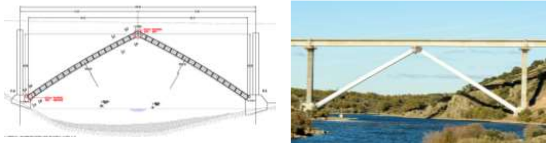
Figure 6. Arch elevation
