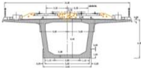
Figure 2. Typical deck cross section
