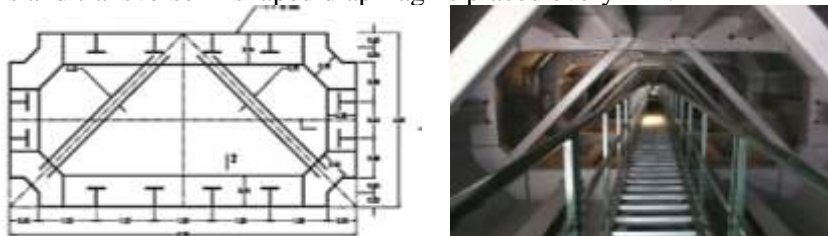
Figure 7. Steel arch cross section
