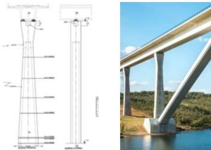
Figure 5. Piers. Elevation and view
